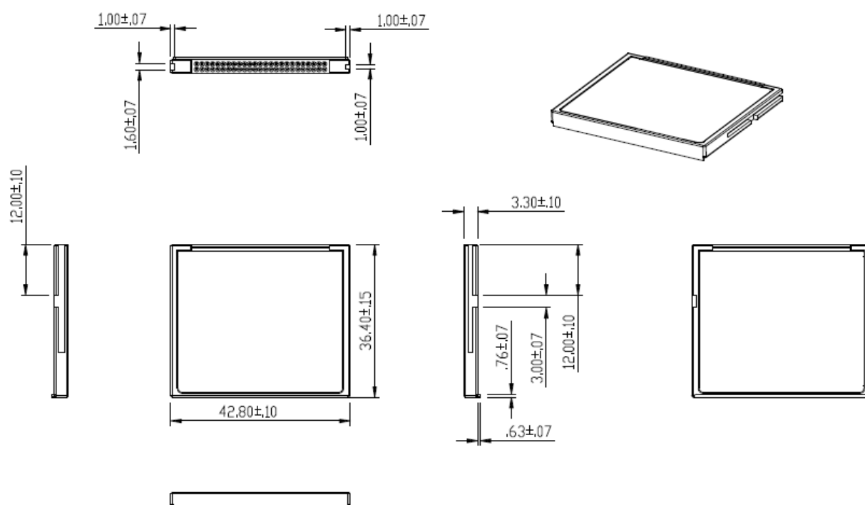
Figure 7-1 Physical Dimensions.
