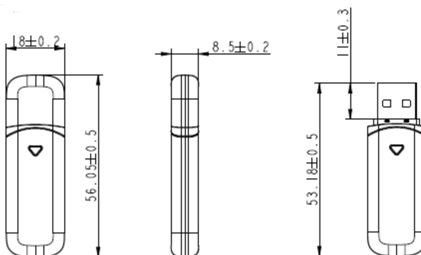
Figure 6-1 Physical Dimensions
