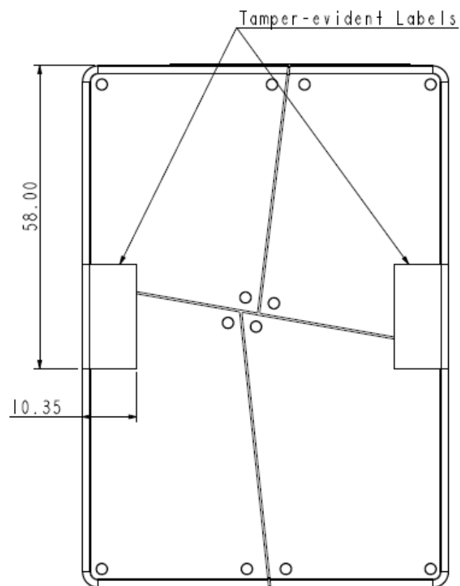
Figure 9-1 Physical Dimensions
