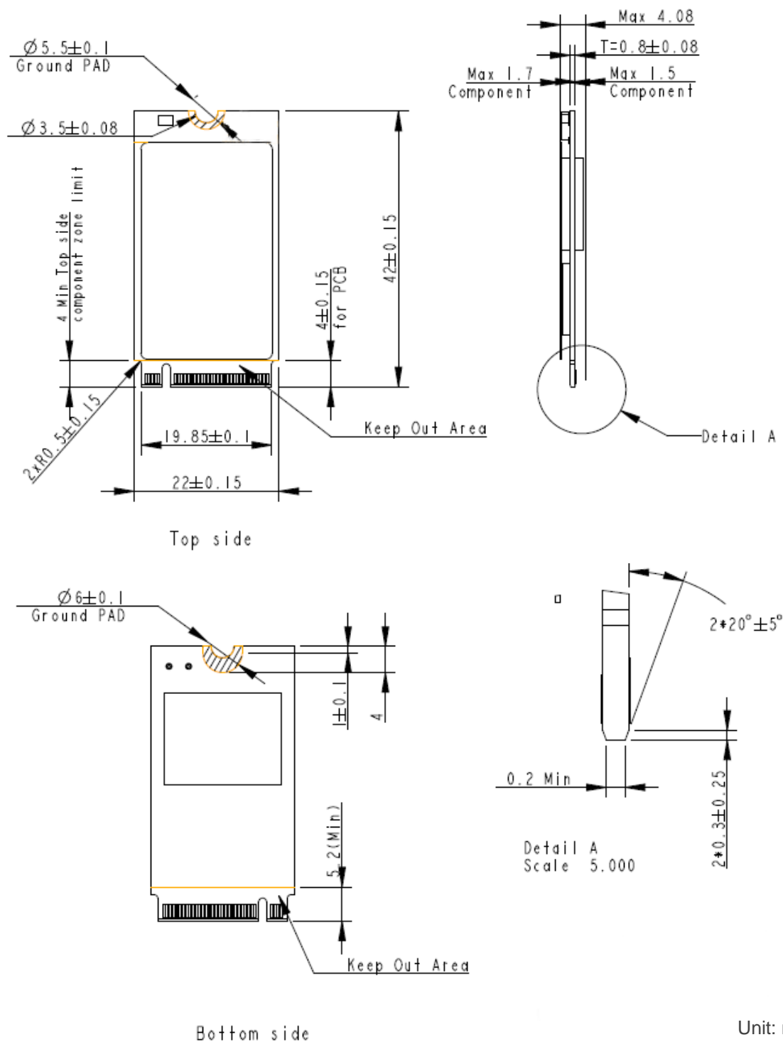
Figure 10-1 Physical Dimensions
