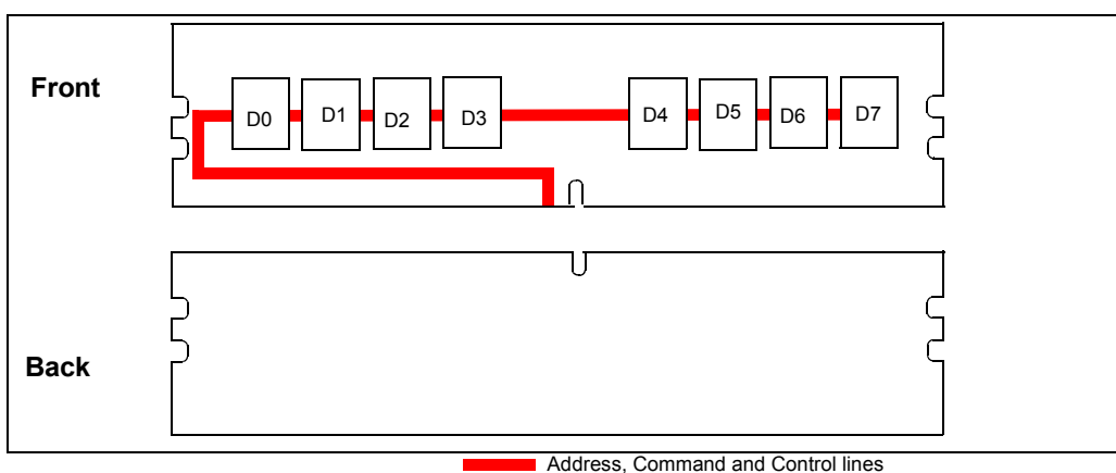
Address, Command and Control lines
