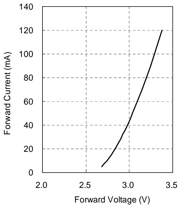
Fig 3. Forward Current
