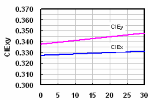
Fig.7. CIExy vs. Forward Current
