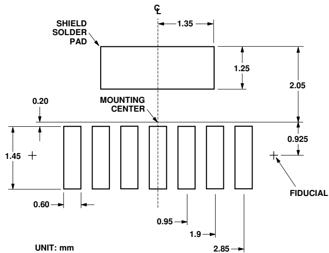
Figure 23. Land Pattern.
