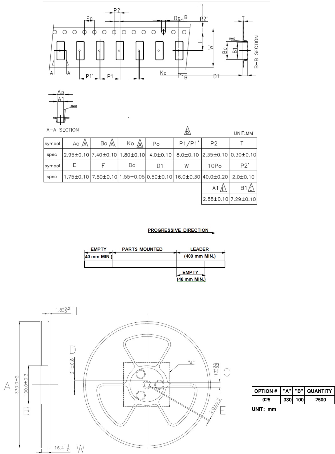
Figure 13. Tape and reel dimensions.
