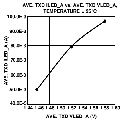
Figure 11. VLED vs. ILED.
