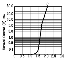
Fig5. FORWARD CURRENT VS. FORWARD VOLTAGE
