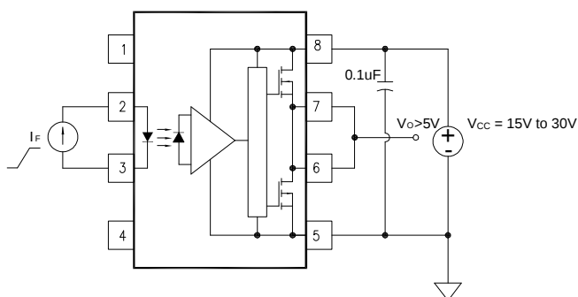
Figure 18 : I_{FH} Test Circuit
