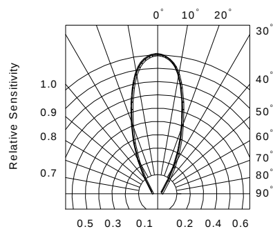
FIG.5 SENSITIVITY DIAGRAM
