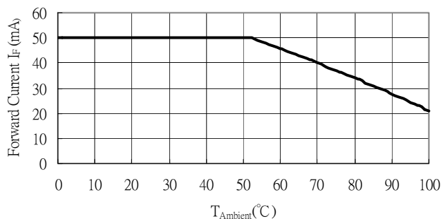
Fig. 3 Forward Current VS Ambient Temperature
