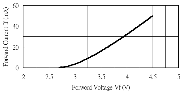
Fig. 2 Forward Current VS Forward Voltage
