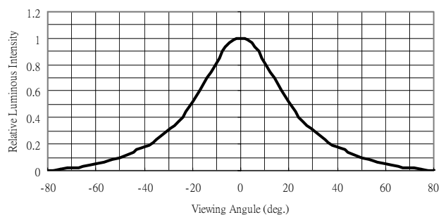
Fig. 5 Relative Intensity VS Off Axis Angle
