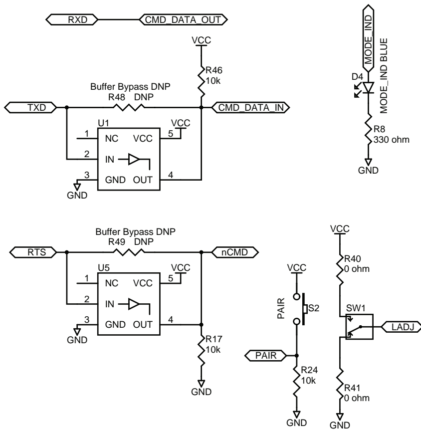
Figure 11: Programming Dock Board Signal Routing Schematic
