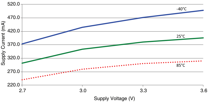
Figure 8: Amplified HumPRO™ Series Transceiver TX Current vs. Supply Voltage at Max Power
