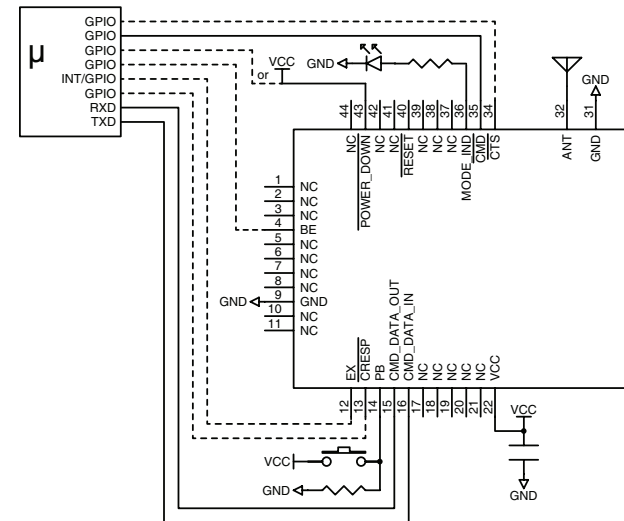
Figure 106: Amplified HumPRO™ Series Transceiver Basic Application Circuit
