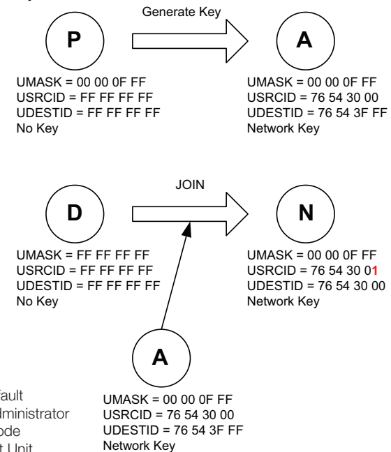
Figure 30: Amplified HumPRO™ Series JOIN Process
