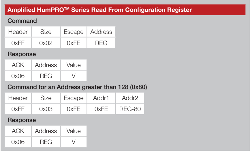
Figure 35: Amplified HumPRO™ Series Read from Configuration Register Command and Response
