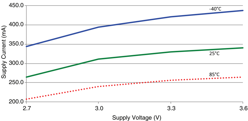
Figure 7: Amplified HumPRO™ Series Transceiver TX Current vs. Supply Voltage at 24dBm
