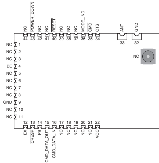
Figure 16: Amplified HumPRO™ Series Transceiver Pre-certified Version Pin Assignments - Castellation Connection (Top View)
