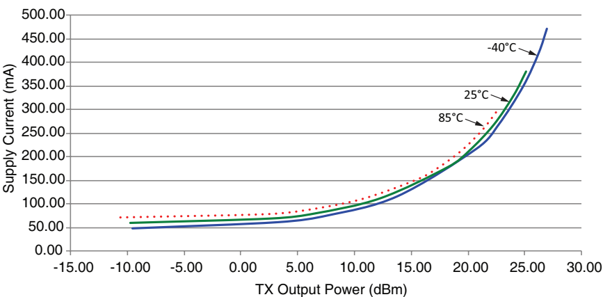
Figure 9: Amplified HumPRO™ Series Transceiver Average TX Current vs. Transmitter Output Power at 3.3V
