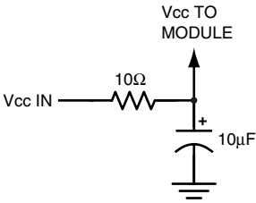
Figure 10: Supply Filter
