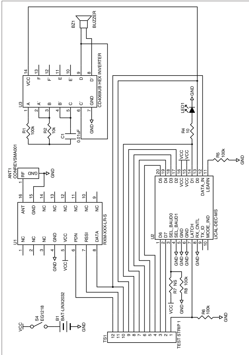
Figure 6: LR Receiver Evaluation Board Schematic
