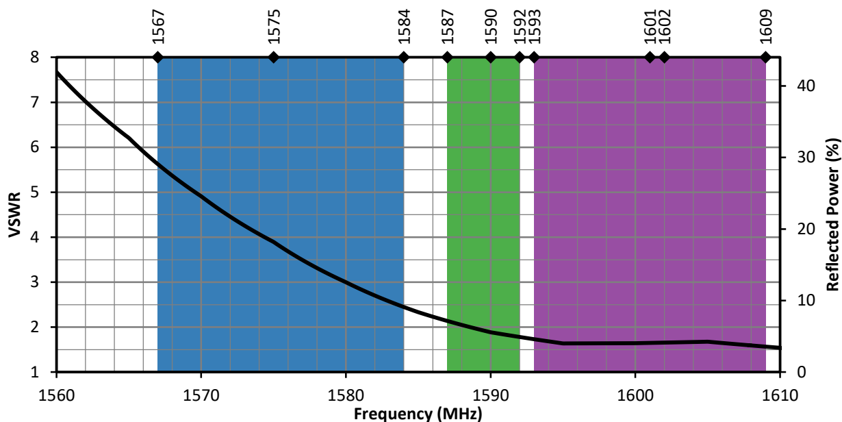
Figure 2. GNSSCP-TH25L1 VSWR
