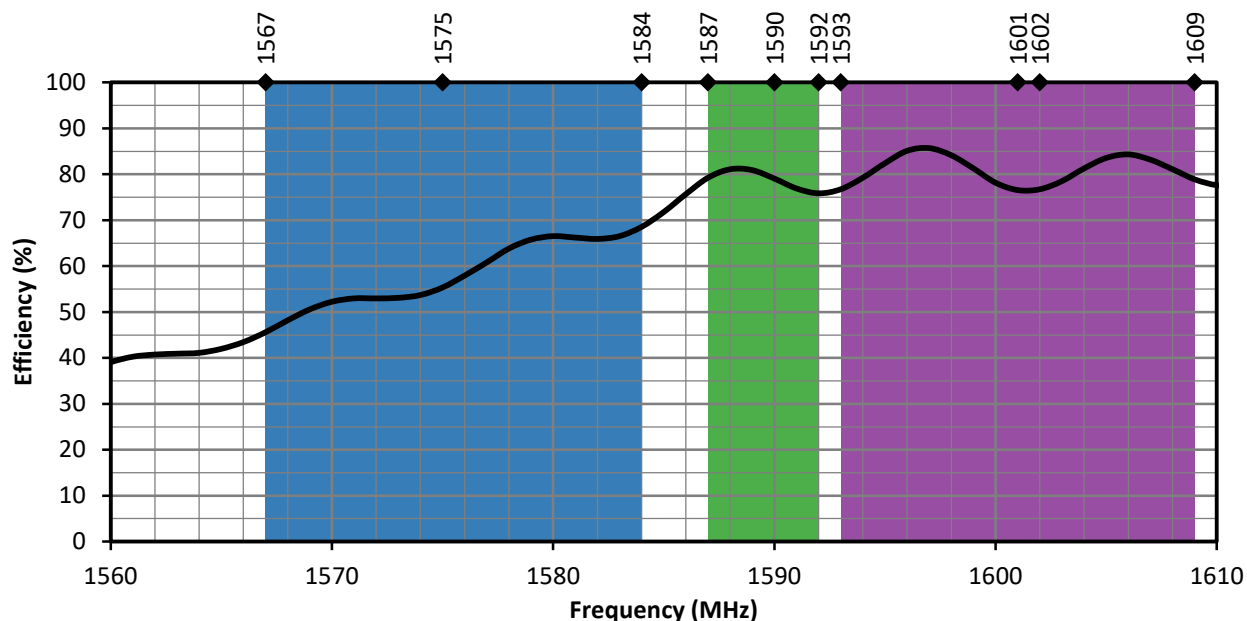
Figure 7. GNSSCP-TH25L1 Antenna Radiation Efficiency
