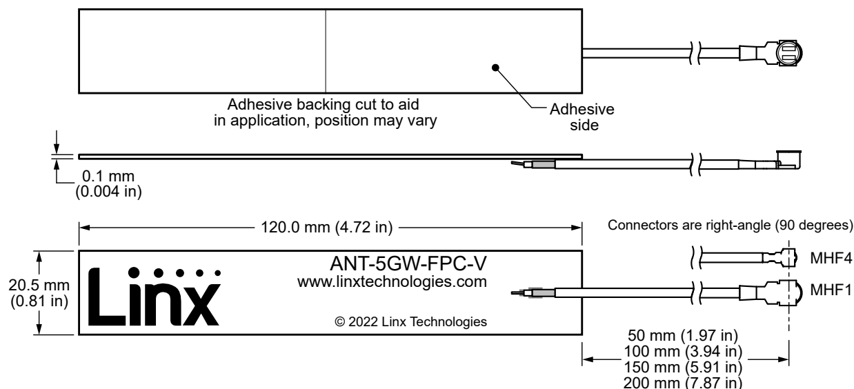
Figure 1. ANT-5GW-FPC-V Series Antenna Dimensions
