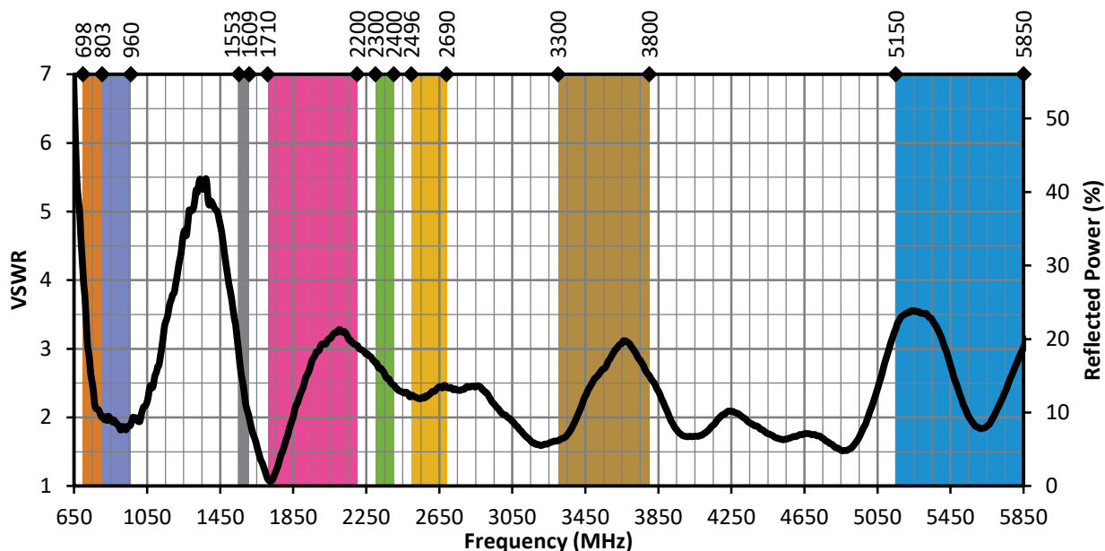
Figure 1. LPX Antenna VSWR with Frequency Band Highlights
