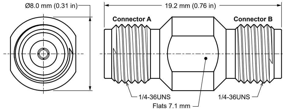
Figure 1. Product Dimensions for the ADP-2.92F-2.92F Adapter
