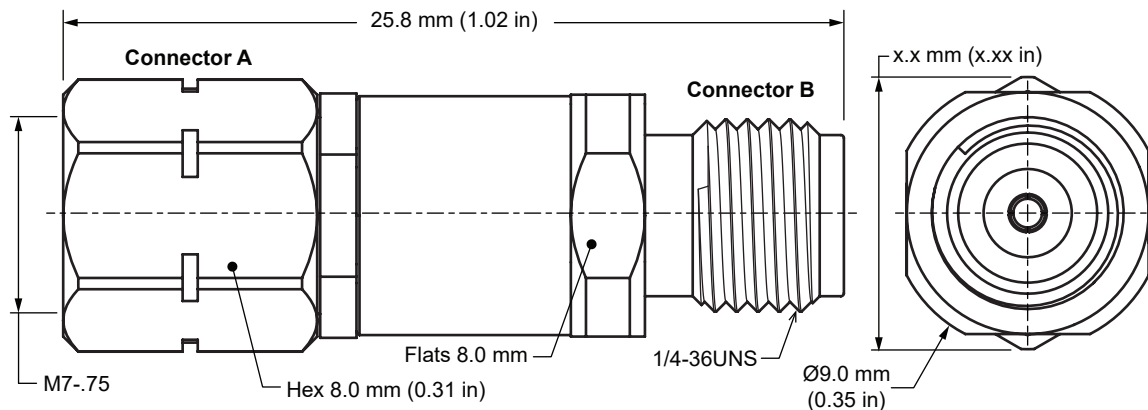
Figure 1. Product Dimensions for the ADP-2.4M-2.92F Adapter
