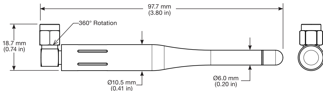
Figure 1. ANT-868-CW-RCL Antenna Dimensions
