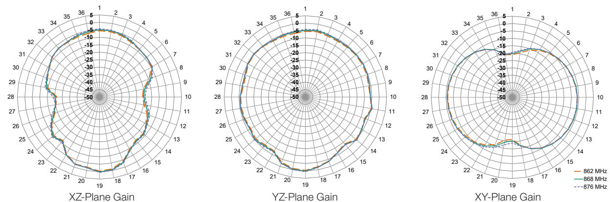
Figure 8. ANT-868-uSP410 Radiation Patterns
