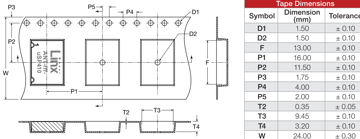
Figure 12. Tape Specifications for the uSP410 Series Antenna
