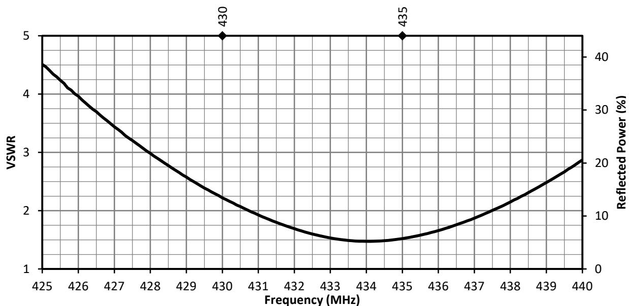
Figure 1. ANT-433-uSP410 VSWR
