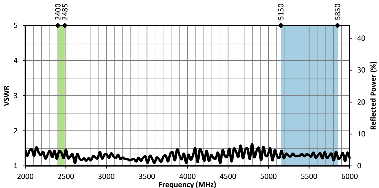
Figure 1. ANT-2/5-HDP-2000 Antenna VSWR, with Frequency Band Highlights
