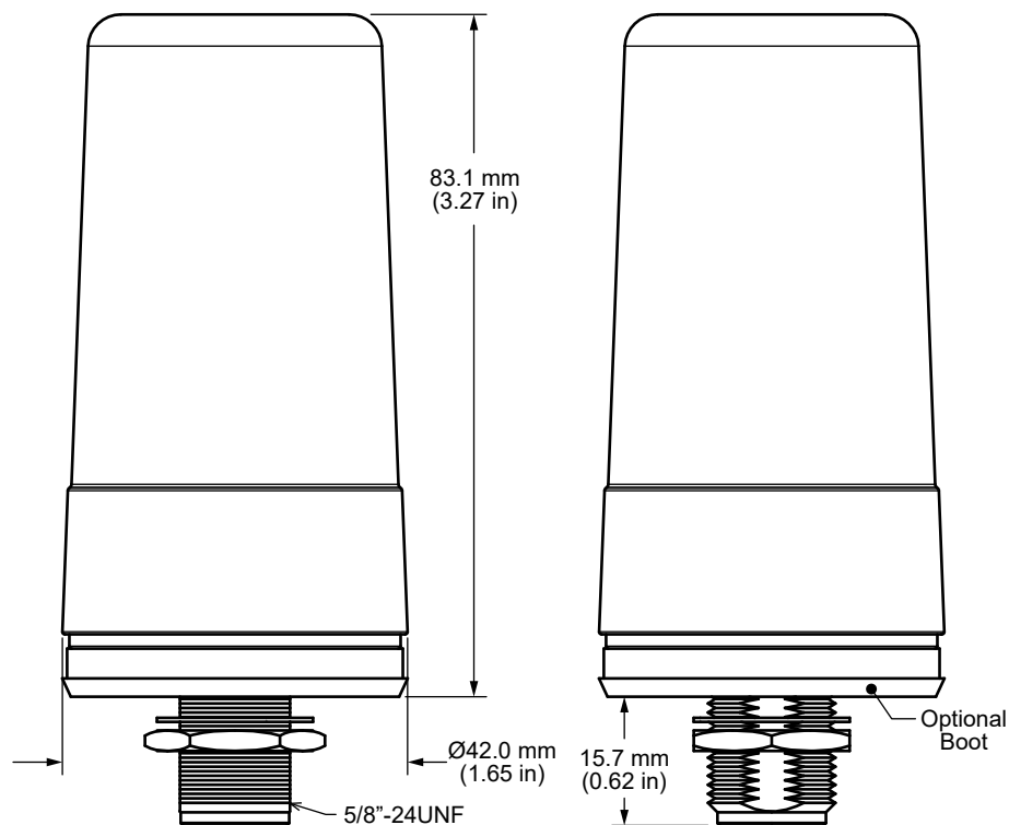
Figure 1. ANT-8/9-SPNF2 Dimensions
