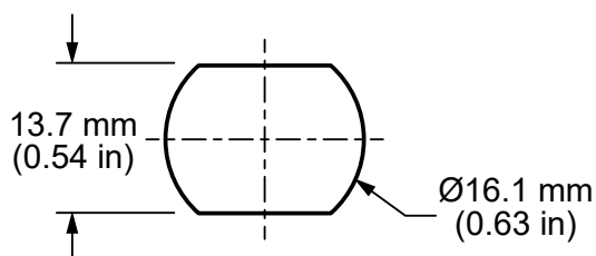
Figure 8. ANT-8/9-SPNF2 Mounting Hole Dimensions
