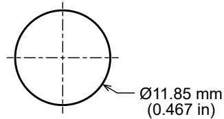
Figure 8. ANT-433-SPS1 Mounting Hole Dimensions
