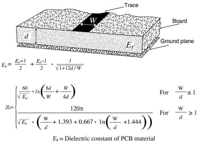
Figure 97: Microstrip Formulas
