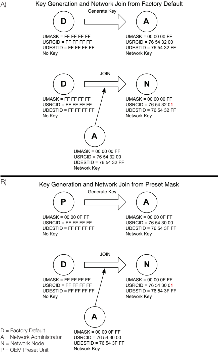
Figure 23: HumPRC™ Series and HumPRO™ Series Join Process Examples
