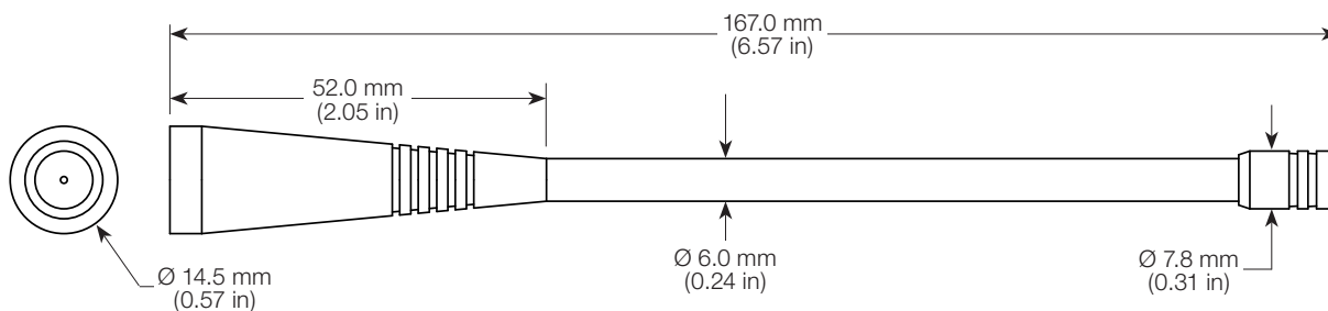
Figure 6. CW 450 MHz Antenna Dimensions
