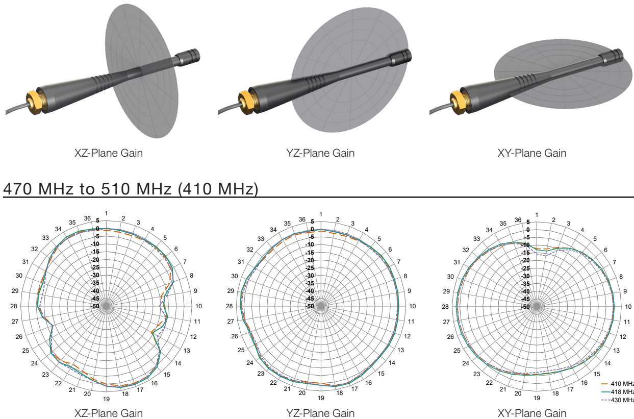
Figure 8. Radiation Patterns for PW 410 MHz Antenna
