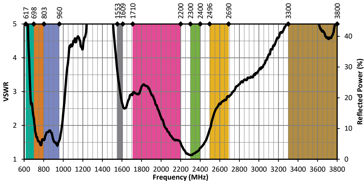
Figure 3. MON-E VSWR, with Frequency Band Highlights
