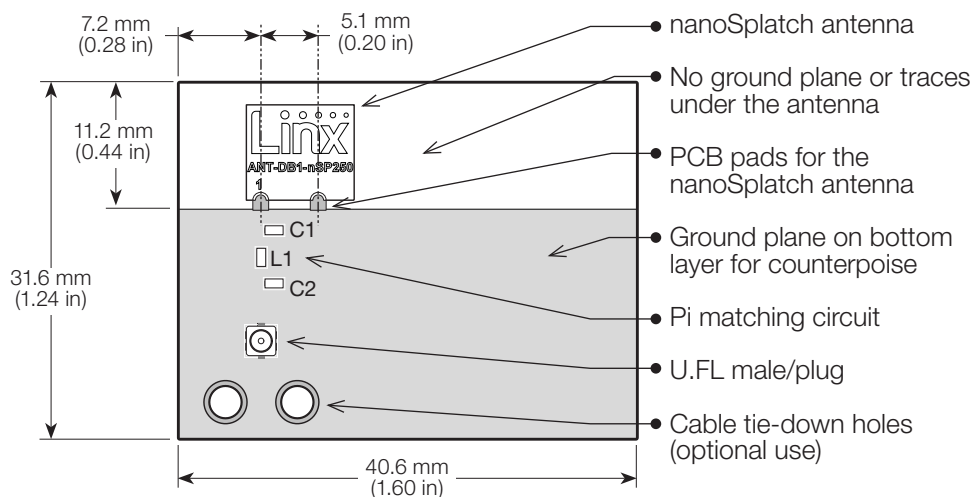
Figure9. Linx nSP250 Recommended Layout
