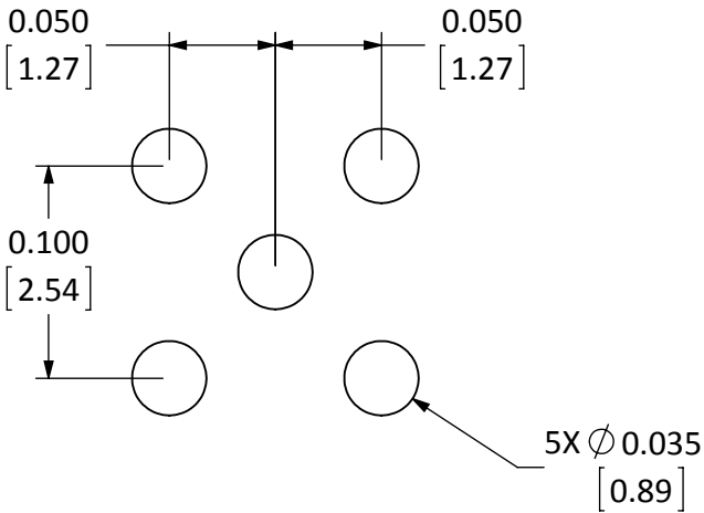
RECOMMENDED FOOTPRINT
