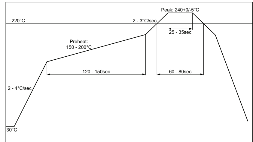
Figure 55: Maximum Reflow Temperature Profile
