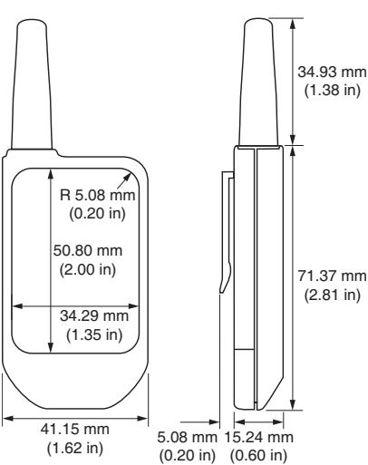
Small Package
