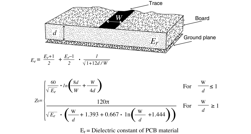
Figure 20: Microstrip Formulas
