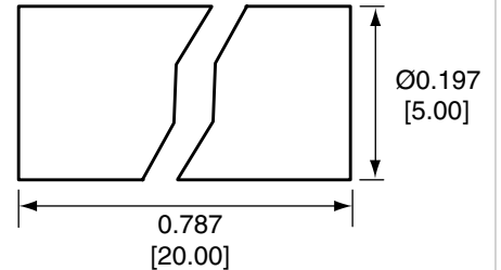
HEAT SHRINK
