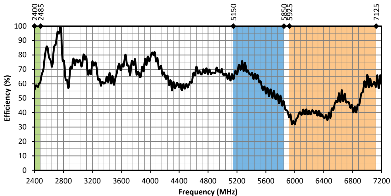
Figure 8. ANT-W63-IPW3-NP Series Antenna Radiation Efficiency, Free Space
