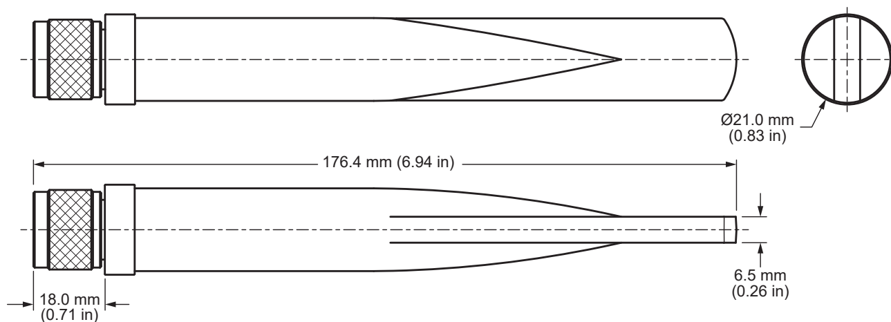
Figure 1. ANT-W63-IPW3-NP Antenna Dimensions
