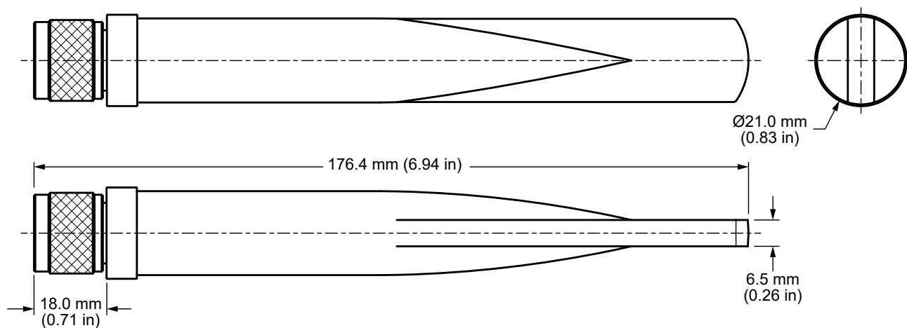
Figure 1. ANT-8/9-IPW3-NP Antenna Dimensions
