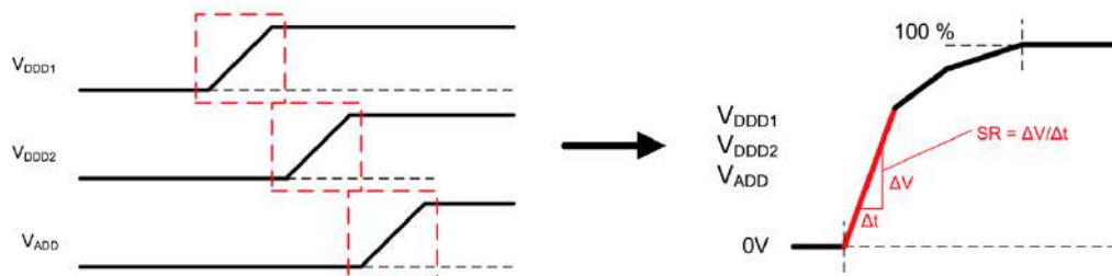
Slew rate of power supply
