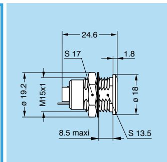
ENG.2B.514 Fixed socket with earthing tag, nut fixing, key (G) or keys (A...F)
