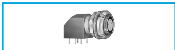
EXG.2B.514 Elbow (90°) socket for printed circuit with two nuts, key (G) or keys (A...F) (back panel mounting)
