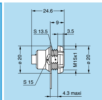
EEG.2B.514 Fixed socket, nut fixing, key (G) or keys (A...F) (back panel mounting)
