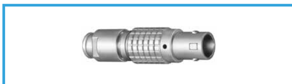
FGG.2B.514 Straight plug, key (G) or keys (A...F), cable collet and nut for fitting a bend relief
