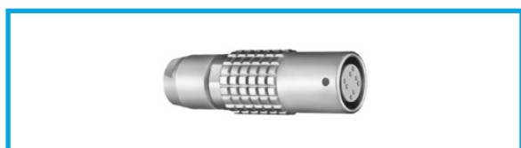
PHG.2B.514 Free socket, key (G) or keys (A...F), cable collet
