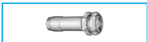
PFG.2B.514 Fixed socket, with two nuts, key (G) or keys (A...F), cable collet (back panel mounting)
