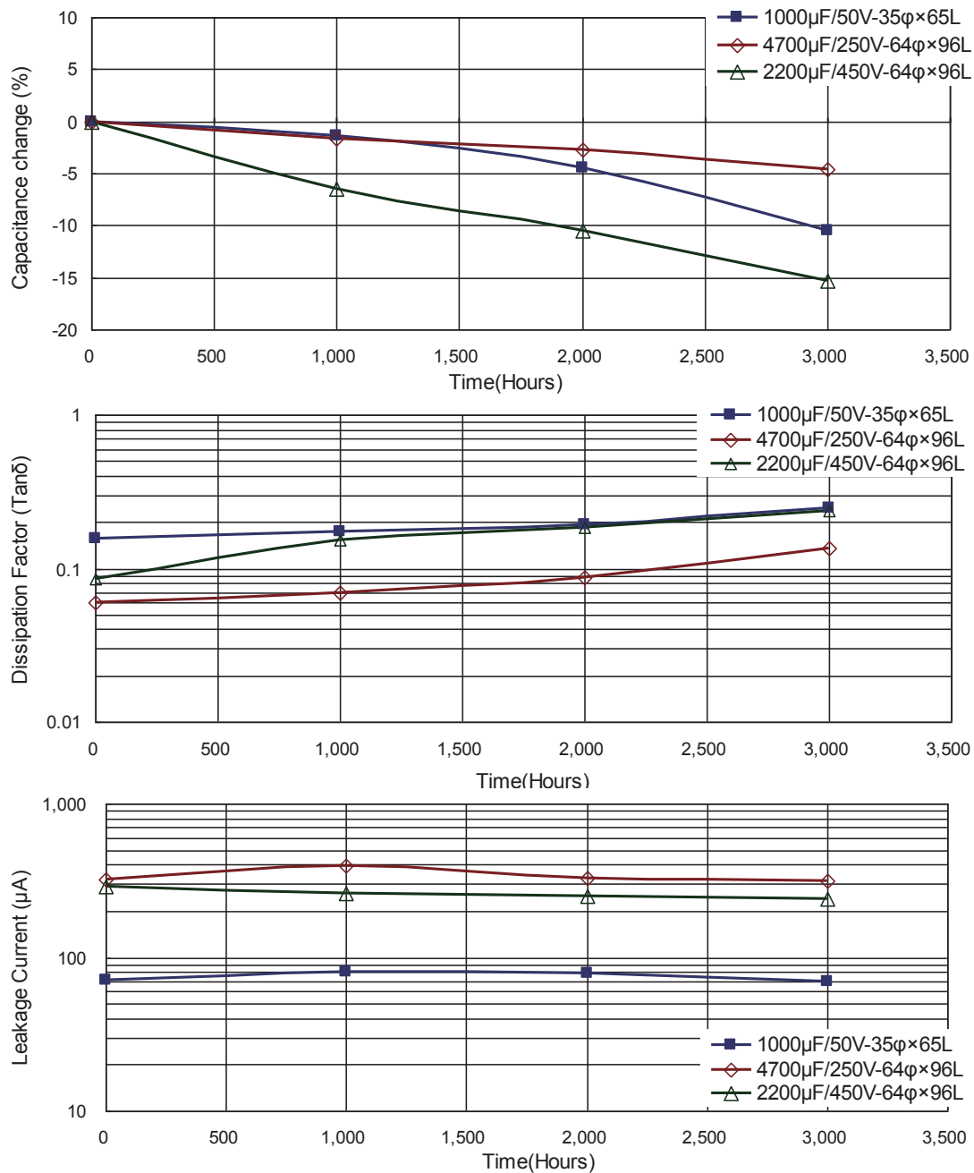
Useful Life Chart
