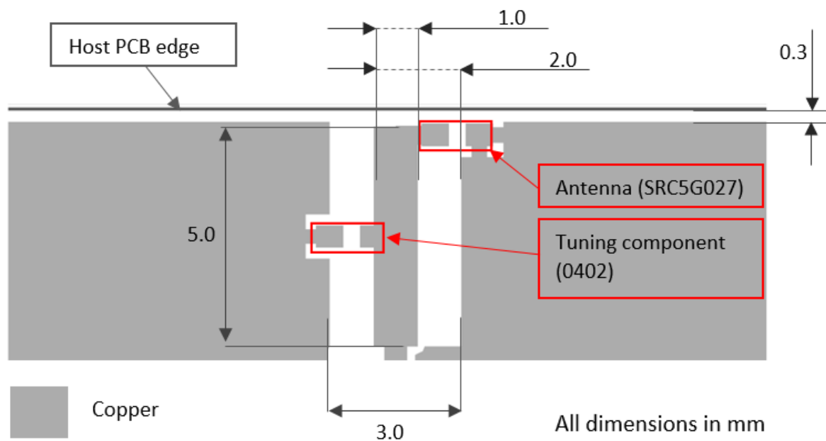
SRC5G027 PCB layout
