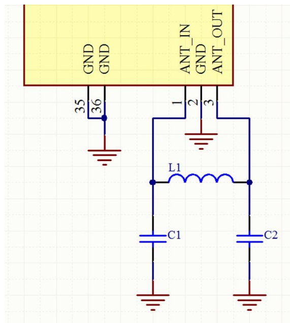
External matching circuit schematic Low-pass configuration
