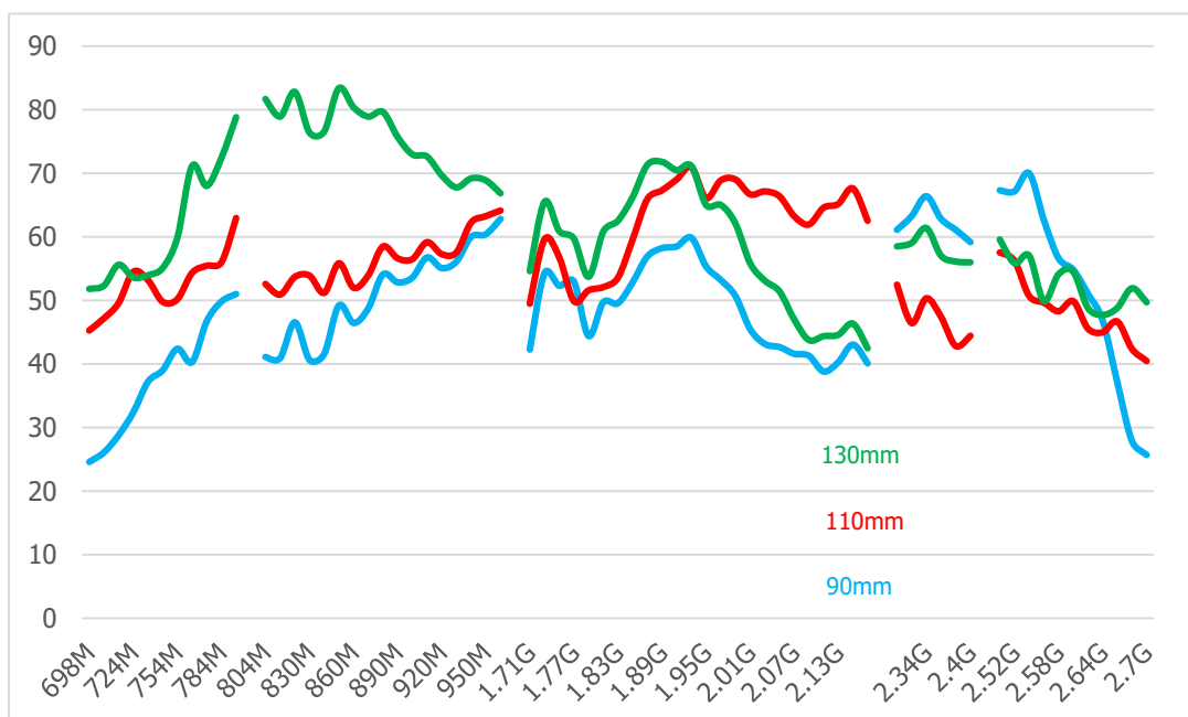
Passive Efficiency vs. PCB length All results measured in Antenna's anechoic chamber
