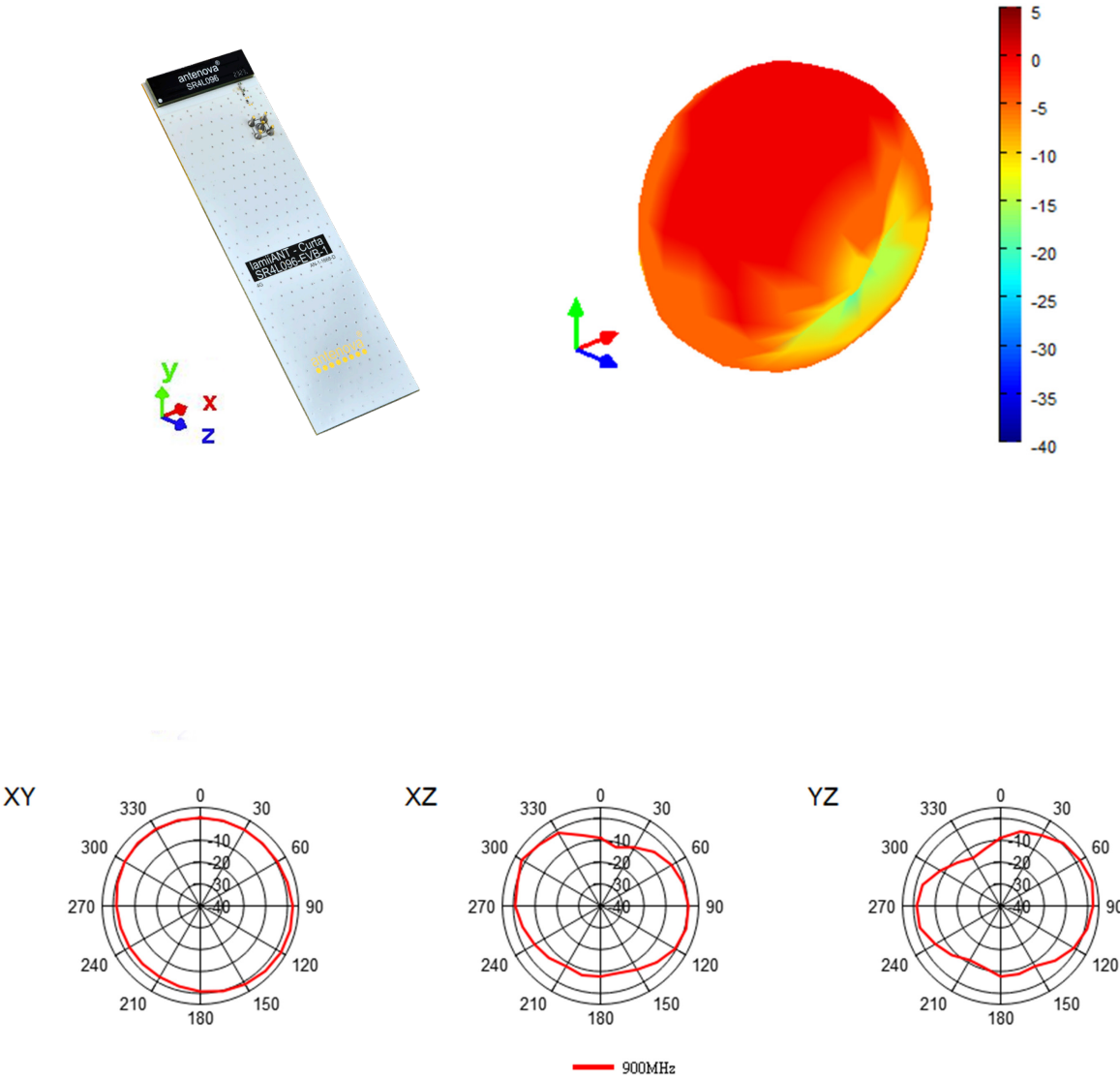
3D pattern at 900MHz
