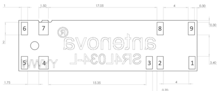
Bottom view
