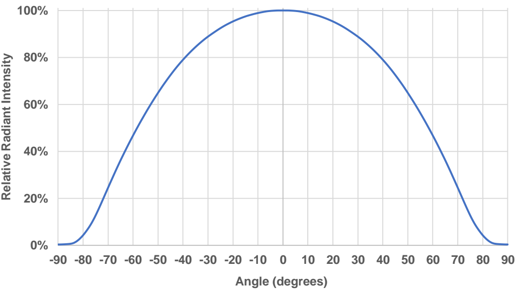
Figure 4: Typical representative spatial radiation pattern
