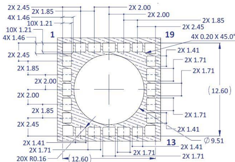
Figure 2b: Recommended Solder Mask Openings (based on Recommended Exposed Minimum Land Pattern)
