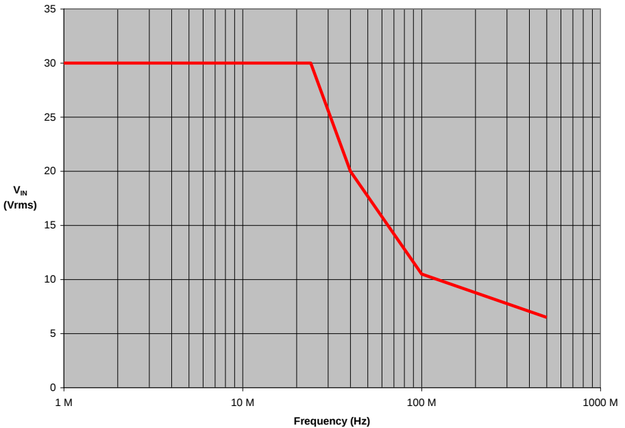
Max. V_{IN} versus Frequency
