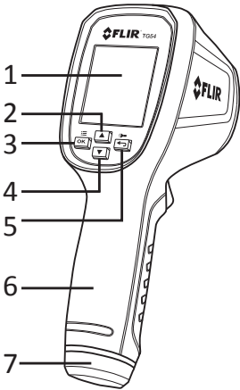
Fig 4-1 Rear View
